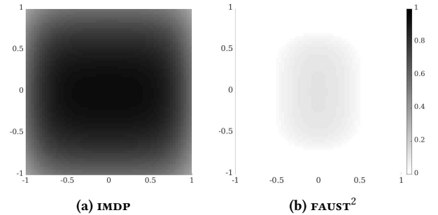
Figure 3: Lower bound probabilities of satisfying \phi_1 with |Q| = 3721 and k = 2 .
